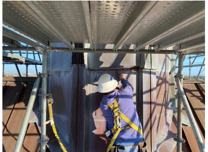
Photo12: Copper Cladding Removed from Base of Steeple
