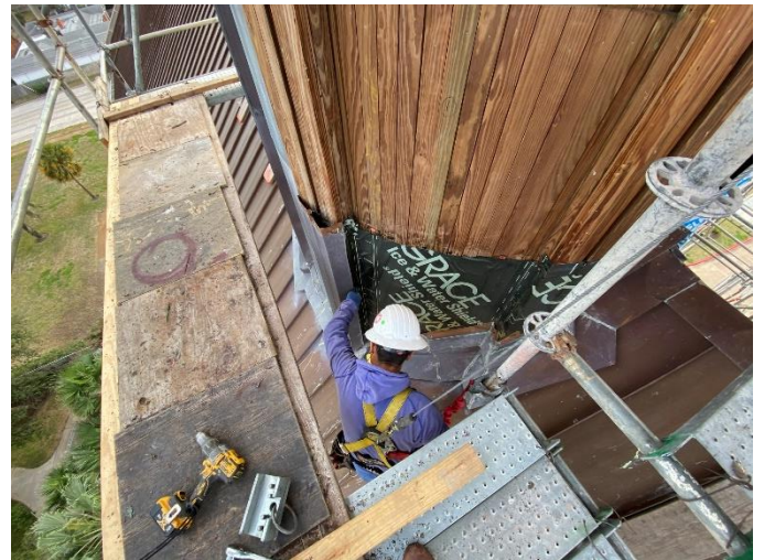
Photo18: Old Membrane Removed
