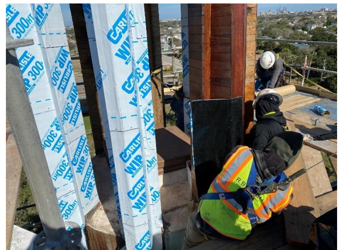
Photo10: Waterproofing Applied
